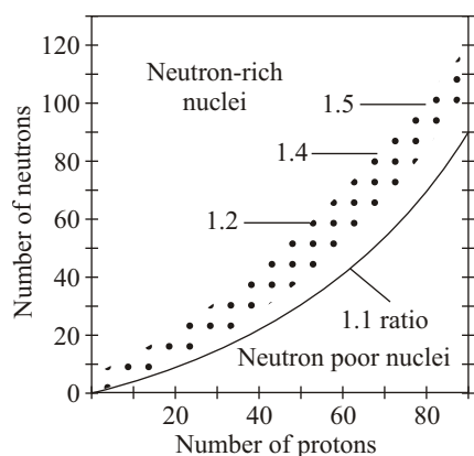
Plot of the number of neutrons against the number of protons in stable nuclei (shown by dots).
