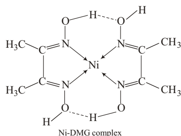
Ni-DMG complex
