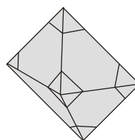
Truncated octahedron
